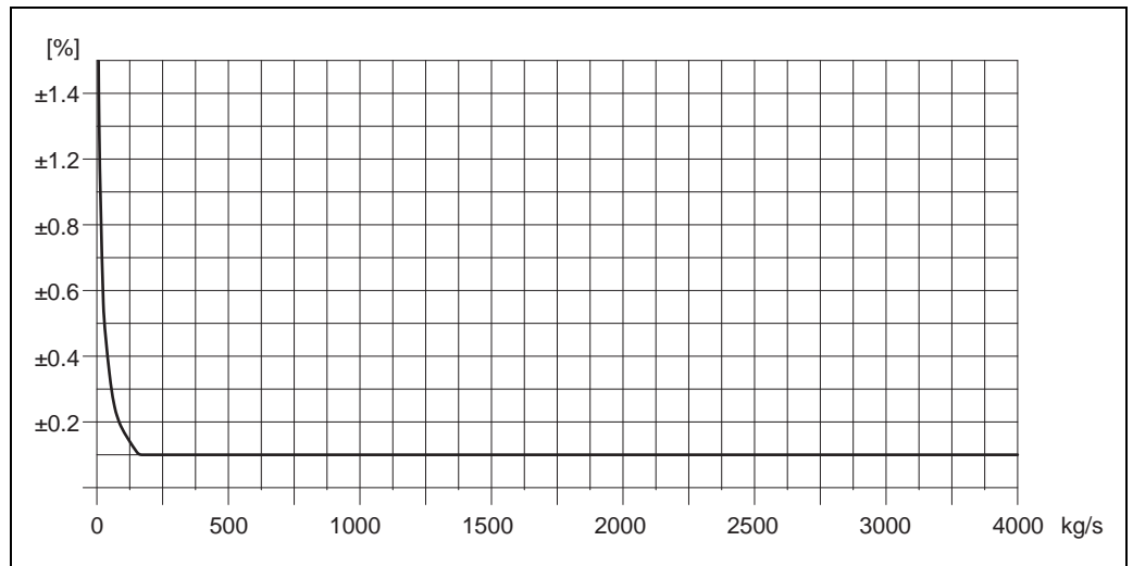
Max. measured error in % o.r. (example: Promass X, DN 350)
